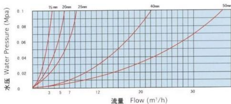
Head Loss Curve
